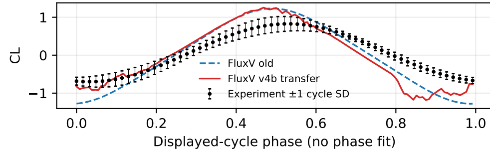
Fig. 14: pitch lagging, U=6 m/s, f=1.5 Hz
