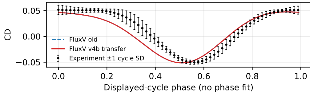
Fig. 9: pitch leading, U=6 m/s, f=0.79 Hz
