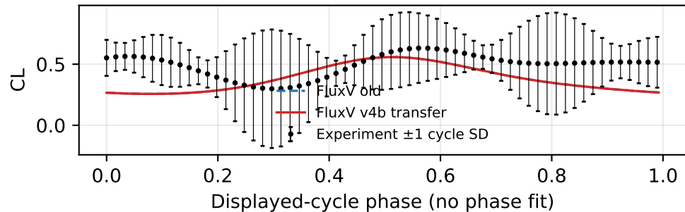
Fig. 9: pitch leading, U=6 m/s, f=0.79 Hz
