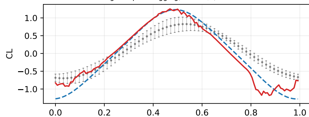
Fig. 15: pitch lagging, U=6 m/s, f=1.5 Hz
