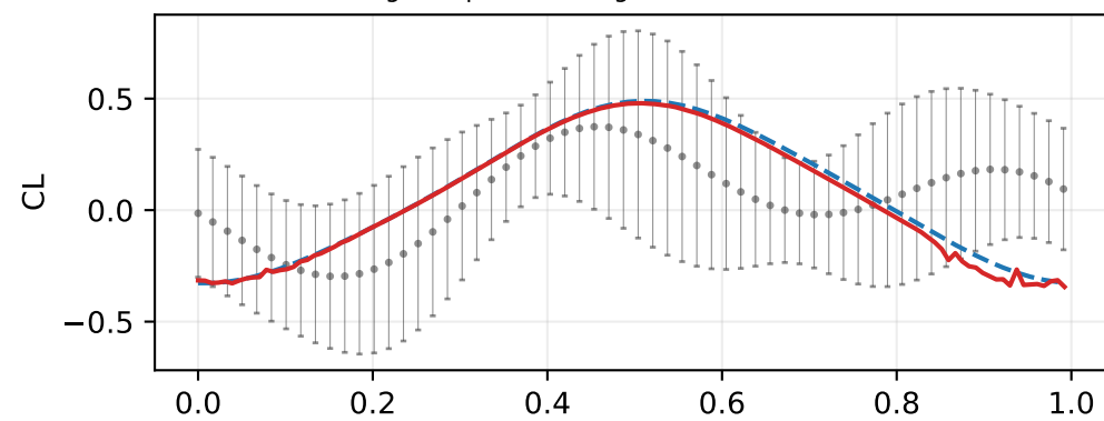
Fig. 11: pitch leading, U=14.8 m/s, f=1.23 Hz
