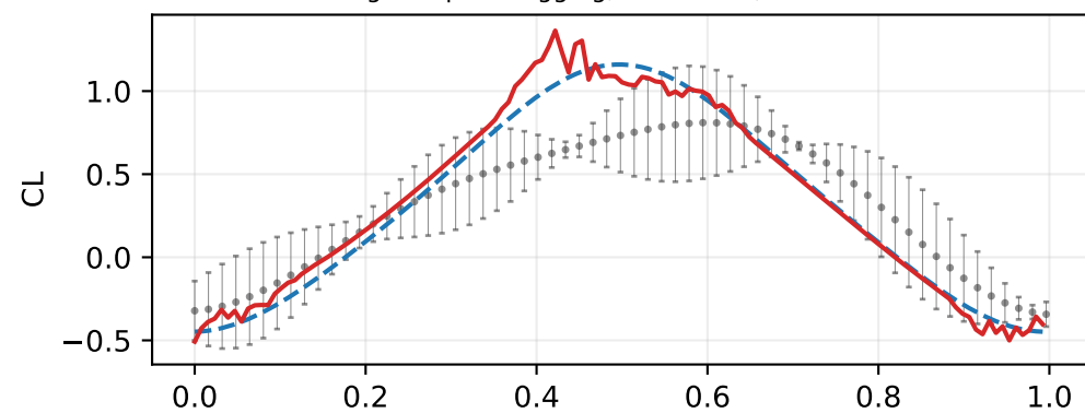
Fig. 14: pitch lagging, U=6 m/s, f=1.5 Hz
