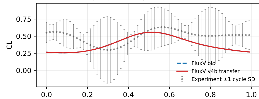
Fig. 10: pitch leading, U=6 m/s, f=1.23 Hz
