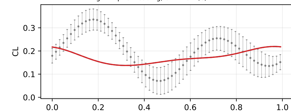
Fig. 13: pitch lagging, U=9.4 m/s, f=1.23 Hz
