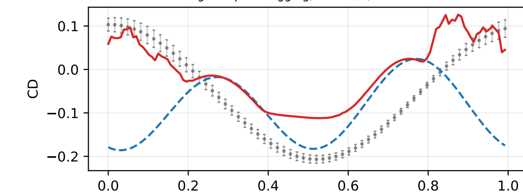
Fig. 15: pitch lagging, U=6 m/s, f=1.5 Hz
