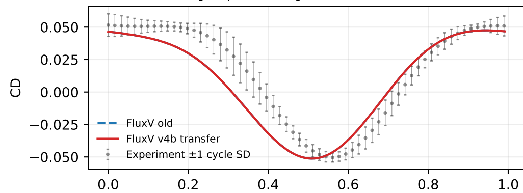
Fig. 10: pitch leading, U=6 m/s, f=1.23 Hz
