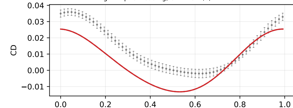
Fig. 13: pitch lagging, U=9.4 m/s, f=1.23 Hz
