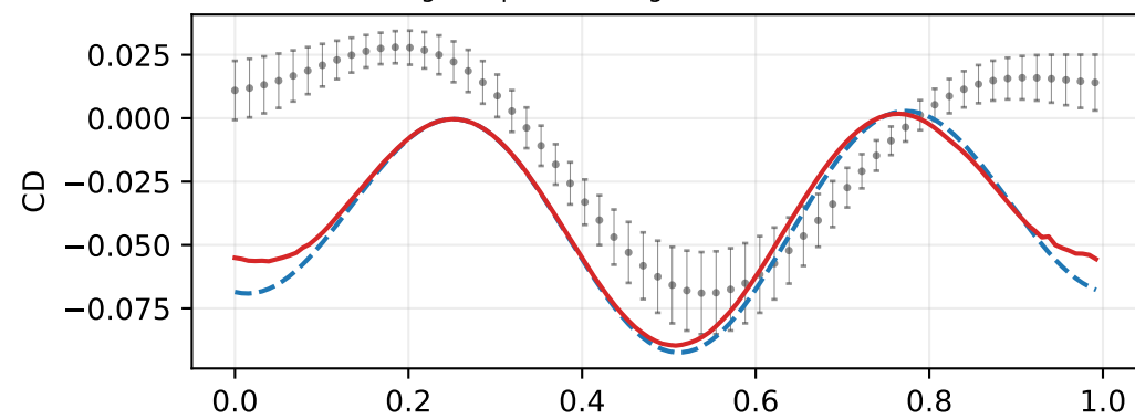
Fig. 11: pitch leading, U=14.8 m/s, f=1.23 Hz
