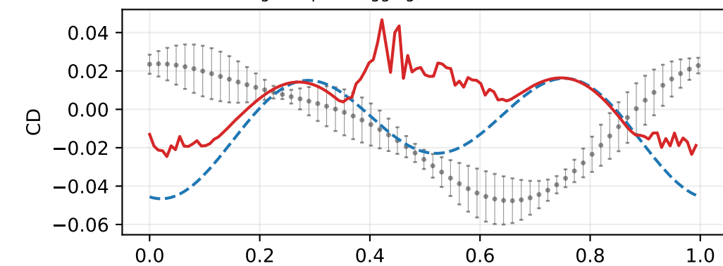
Fig. 14: pitch lagging, U=6 m/s, f=1.5 Hz
