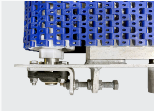
Fig 71 10 threads visible
