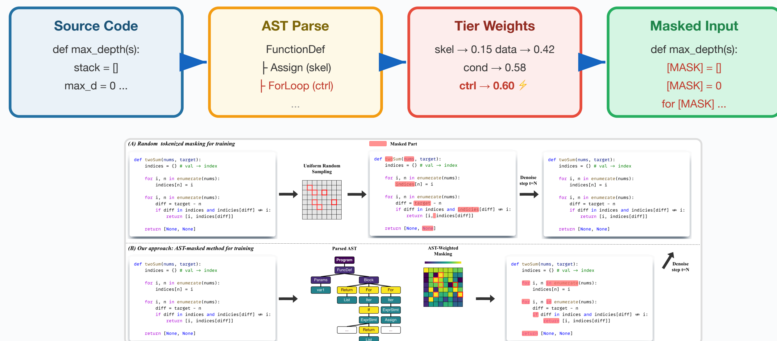
Figure 1: Uniform Random Masking (top) vs. AST-Weighted Sampling Masking (bottom).
