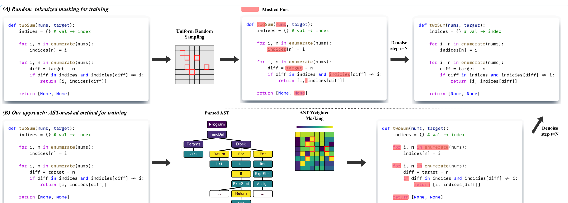
Figure 1: Uniform Random Masking (top) vs. AST-Weighted Sampling Masking (bottom).
