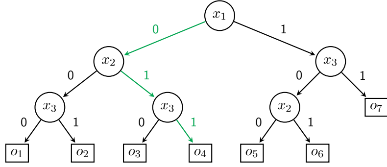
Figure 2. An example of a decision tree of size 13 and depth 3. The green path shows the computation made for the input x = 011 .
