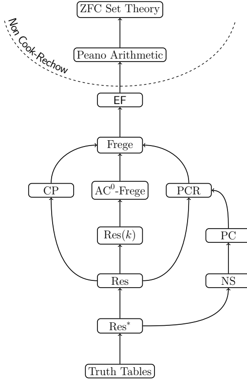
Figure 5. Hierarchy of common proof systems. Omitted arrows imply non p -simulation.
