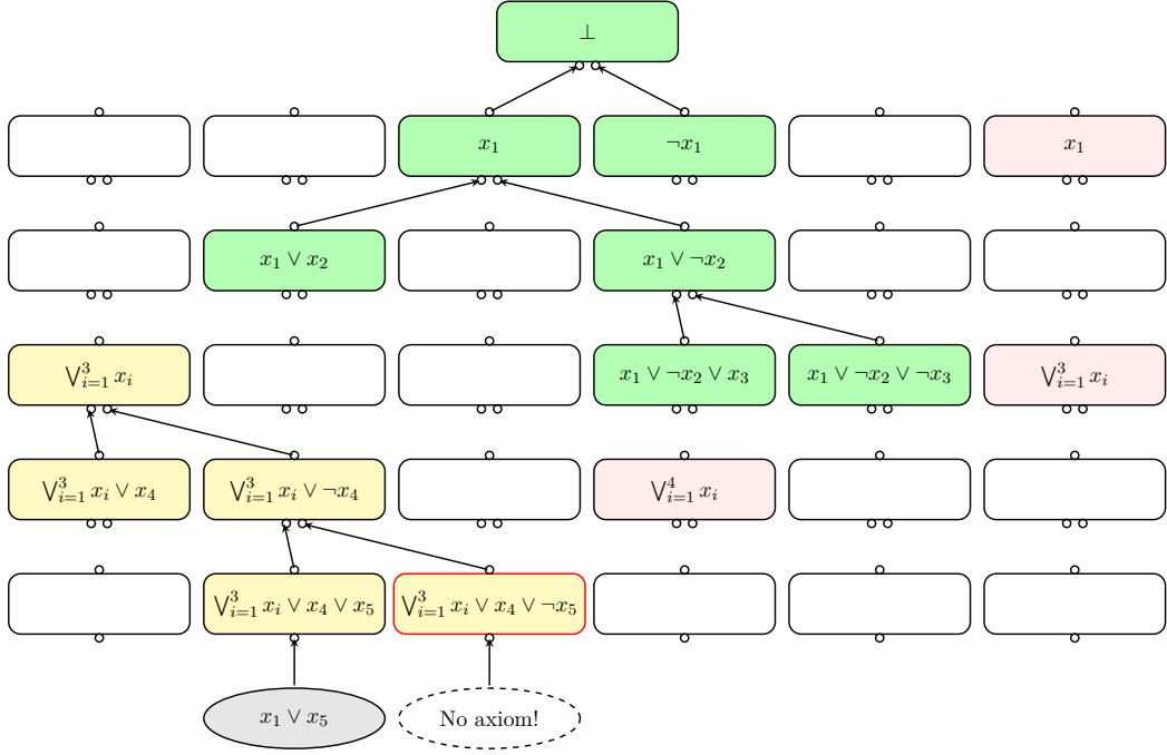
Figure 8. Snapshot of the reservations made during an execution of Algorithm 3 . The green tree is obtained by the answers given by the Duplicator by consistently following the canonical exponential-size tree-like, starting from the root. The yellow tree is obtained in the same way, but starting from an new block that was never mentioned. Pink nodes are queried out-of-context only once. Gray nodes are axioms of \varphi obtained by answering valid weakening steps. The leaf marked in red is not the weakening of any axiom, meaning that its negation is a satisfying assignment.
