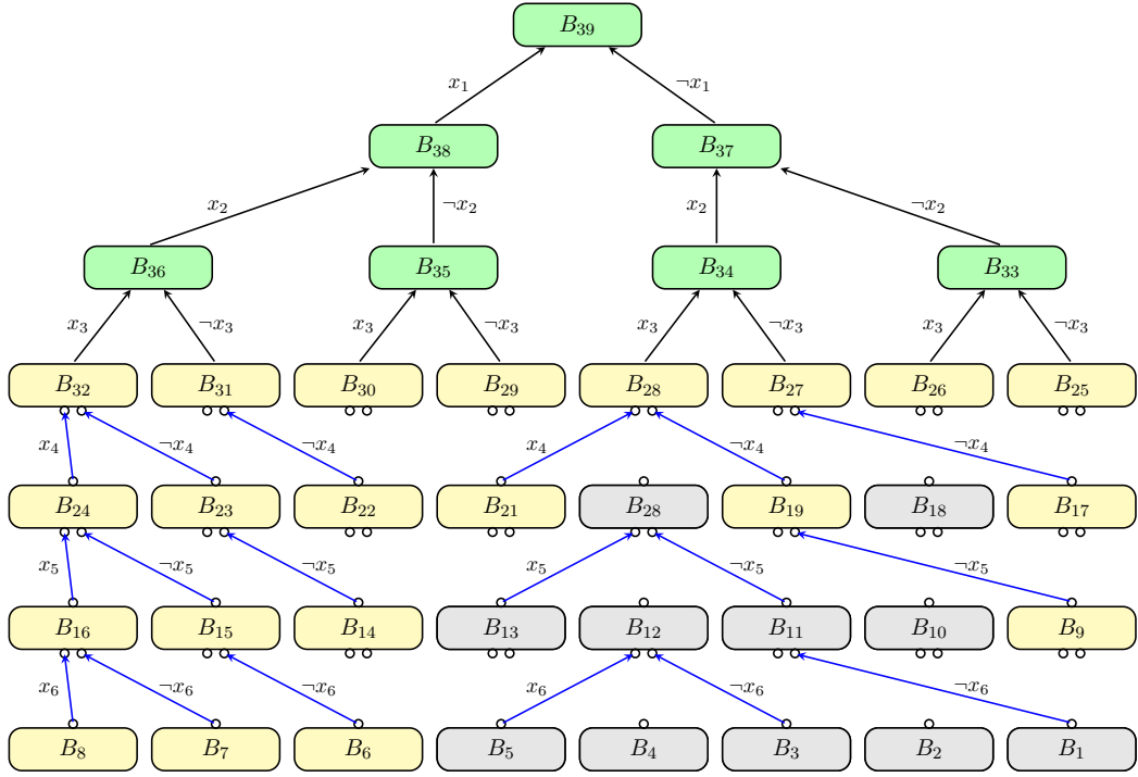
Figure 7. The graph G_\alpha of the reduction from \text{rPHP}_m^{2m} to \text{Ref}_{m(n-\log m+2)-1}(\varphi) with n = 7 and m = 8 . The copies of the partial matching defined by h : [2m] \rightarrow [m] are represented by blue arrows. Hardcoded nodes are represented in green. Derived nodes that survive the walk-up phase are represented in yellow, while disabled blocks are represented in gray. The subtree isomorphic to T_\alpha is given by green and yellow nodes.
