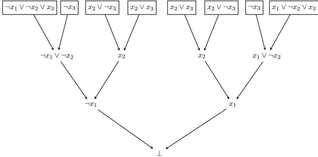
Figure 5. Tree-like adaptation of the refutation in Figure 3.
