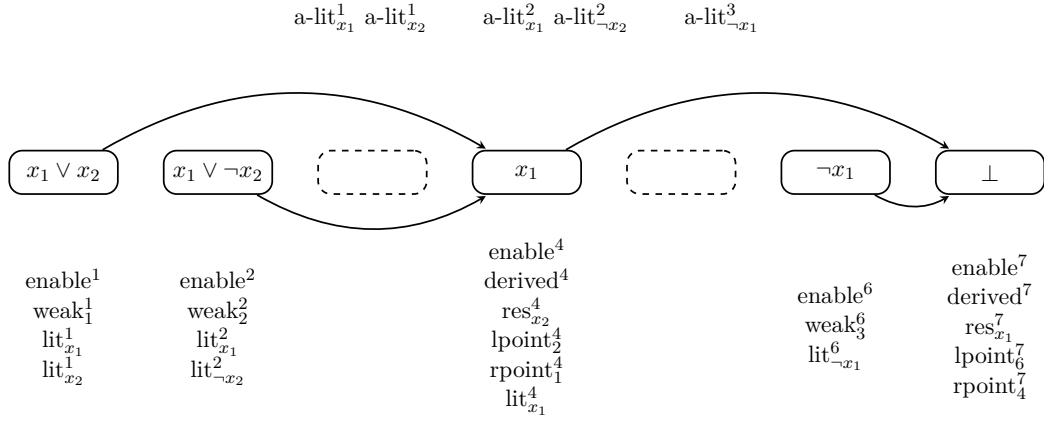
Figure 7. Mapping between a refutation of \varphi = (x_1 \vee x_2) \wedge (x_1 \vee \neg x_2) \wedge \neg x_1 and a satisfying assignment for \text{Ref}_7(\varphi) . Displayed variables are set to 1, the remaining ones are set to 0.
