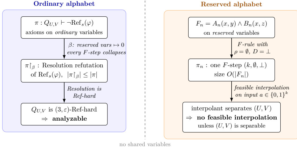
Figure 11. Summary of Lemma 4.26 and Theorem 4.27 .
