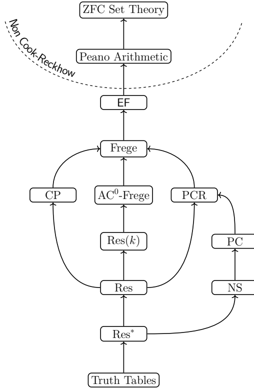
Figure 6. Hierarchy of common proof systems. Omitted arrows imply non p -simulation.
