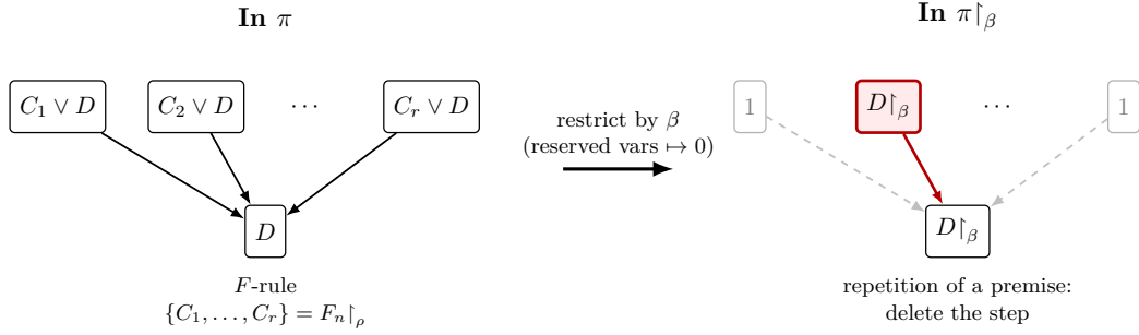
Figure 10. The idea behind Lemma 4.26 . F_n|_\rho is unsatisfiable and all its variables are reserved, so \beta falsifies some clause. That premise becomes D|_\beta , while the other premises become true. Axioms of \text{Ref}_s(\varphi) use only ordinary variables, so \text{Ref}_s(\varphi)|_\beta = \text{Ref}_s(\varphi) .
