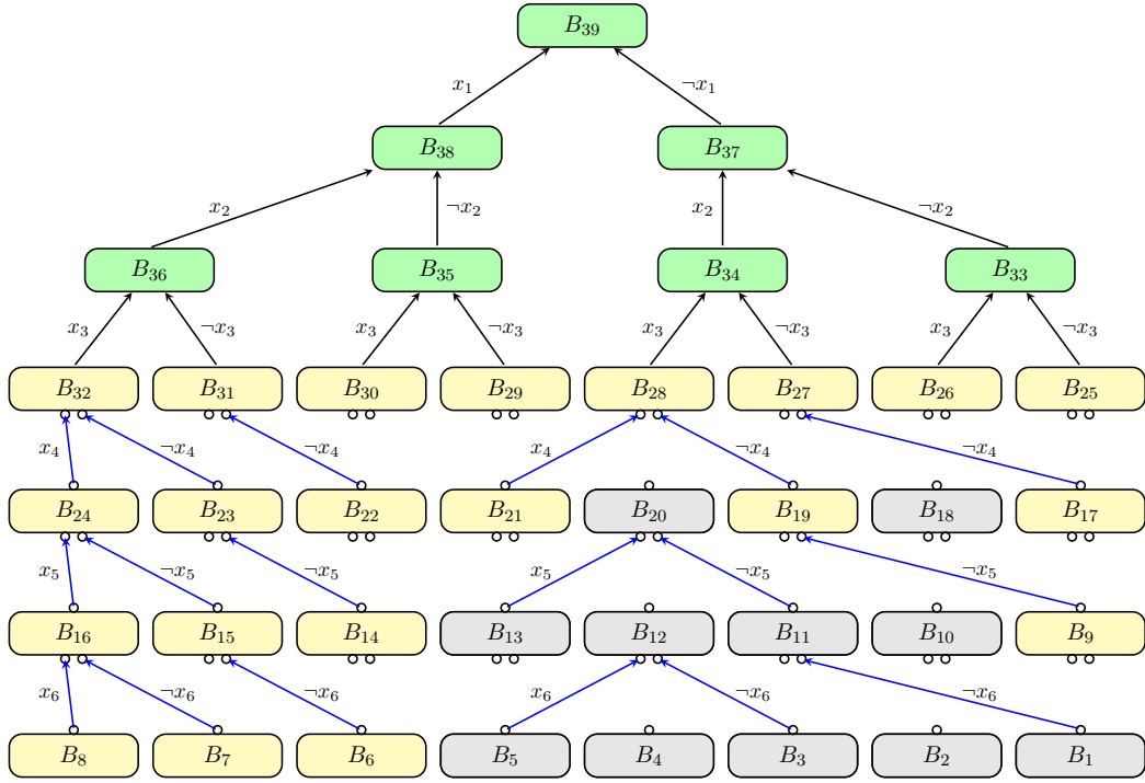
Figure 8. The graph G_\alpha of the reduction from \text{rPHP}_m^{2m} to \text{Ref}_{m(n-\log m+2)-1}(\varphi) with n = 6 and m = 8 . The copies of the partial matching defined by h : [2m] \rightarrow [m] are represented by blue arrows. Hardcoded nodes are represented in green. Derived nodes that survive the walk-up phase are represented in yellow, while disabled blocks are represented in gray. The subtree isomorphic to T_\alpha is given by green and yellow nodes.
