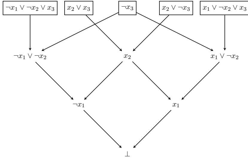
Figure 4. DAG-like representation of the refutation in Figure 3.
