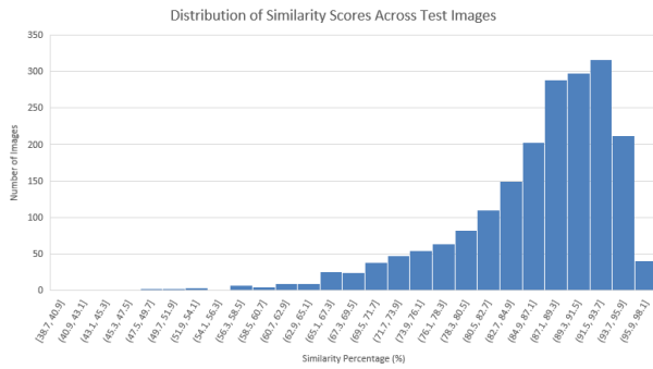
Fig. 6. Histogram of fusion-classifier similarity scores across the test set.
