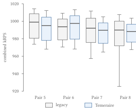
Figure 3: Per-trial combined throughput for the four release-off pairs of the correction run. Boxes span the interquartile range, whiskers the 5th to 95th percentile, and the heavy line the median of 2000 trials. The within-block spread is roughly 4%, an order of magnitude wider than the pairwise deltas in Table 1.
