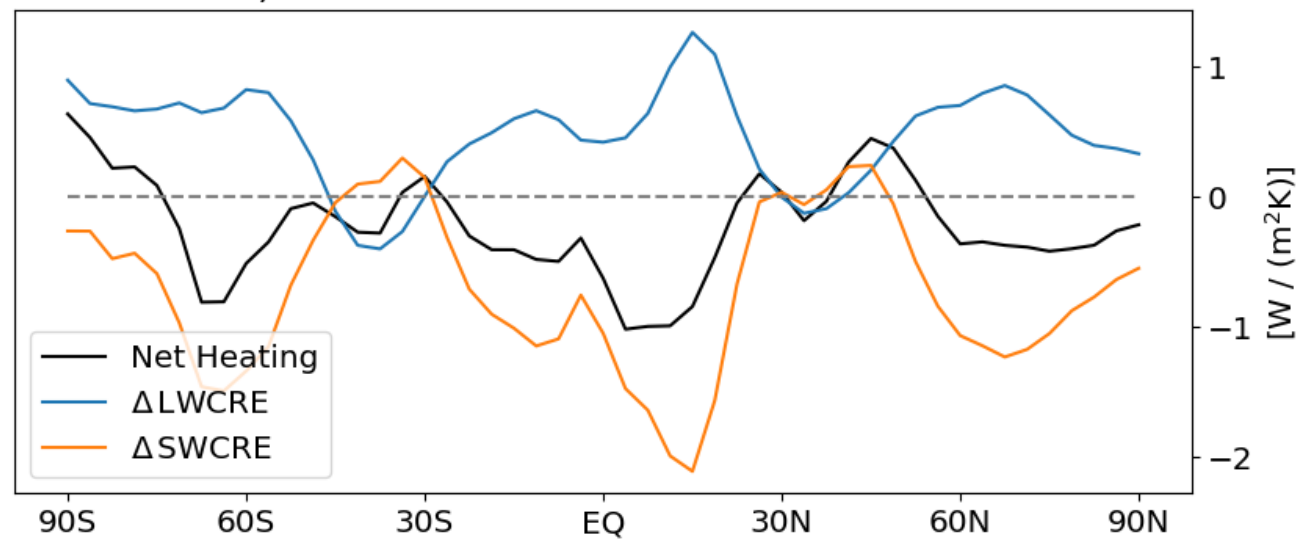
b) Difference in Cloud Radiative Effects
