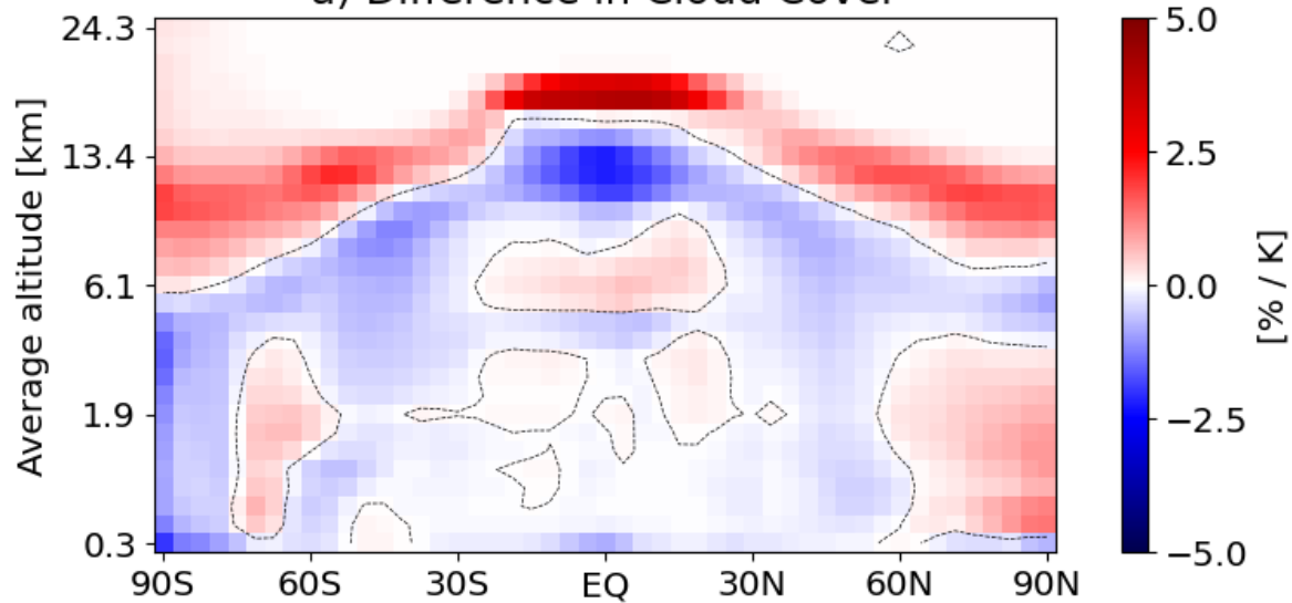
a) Difference in Cloud Cover
