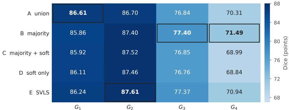
Supervision target
