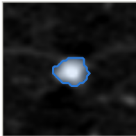
(c) G_1 union
