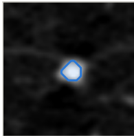
(f) G_4 unanimous
