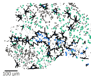
core 6_B: log B rel 1.8, IR +0.5
