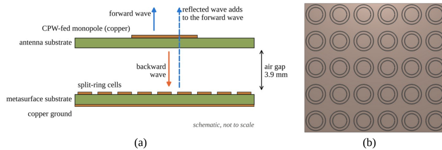
Fig. 1. Proposed structure: (a) side view of the antenna, the 3.9 mm air gap and the metasurface (schematic, not to scale), and (b) CST model of the 6 \times 5 double split-ring metasurface, top view.
