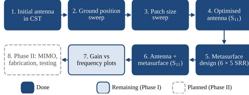
Fig. 2. Design workflow (dark: done; light: remaining in Phase I; dashed: Phase II).
