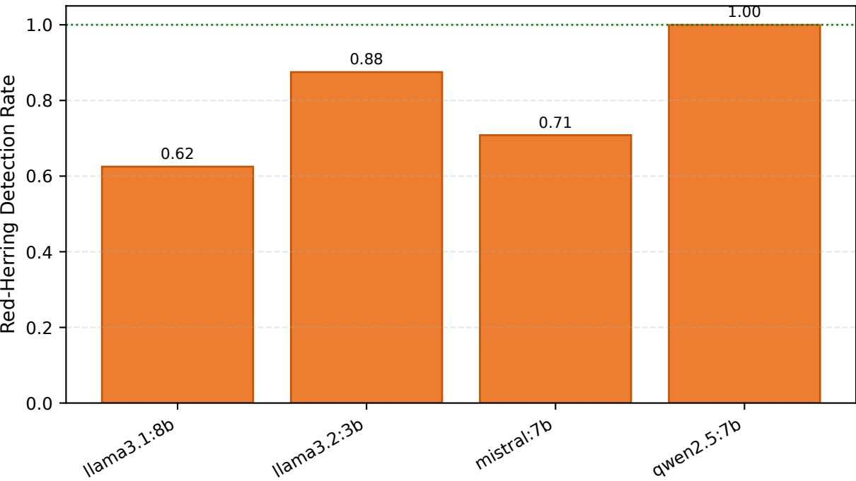
Automation-bias probe (H5): RHDR by model
