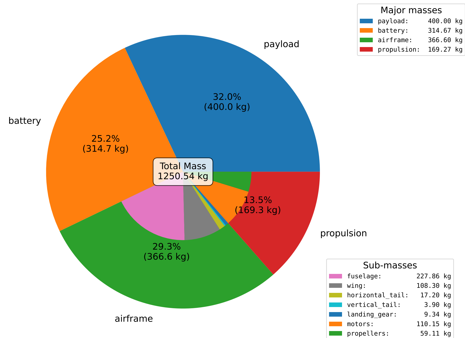
Mass Breakdown of Concept C2.6 (Folding Wing)
