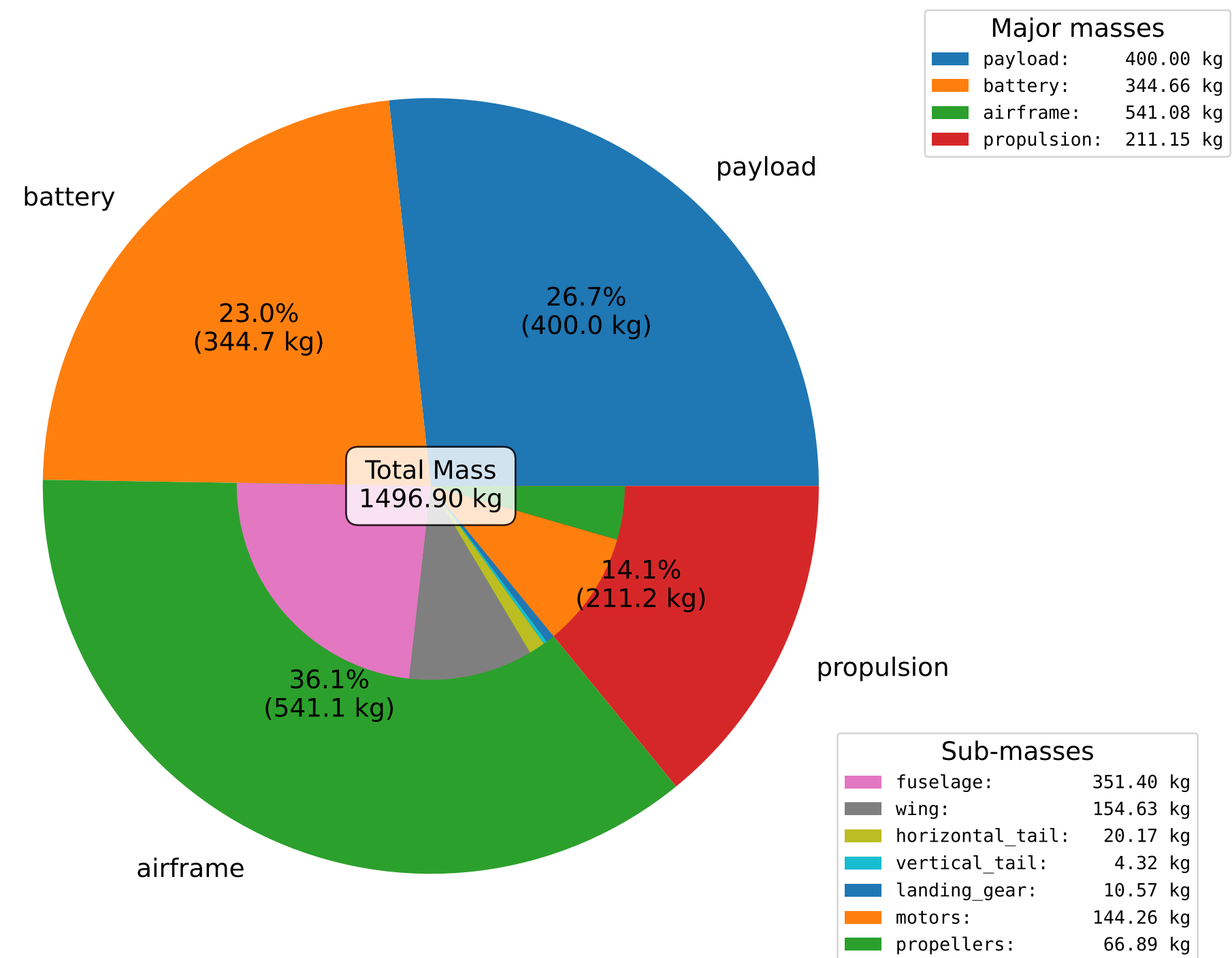
Mass Breakdown of Concept C2.10 (Tomaso)
