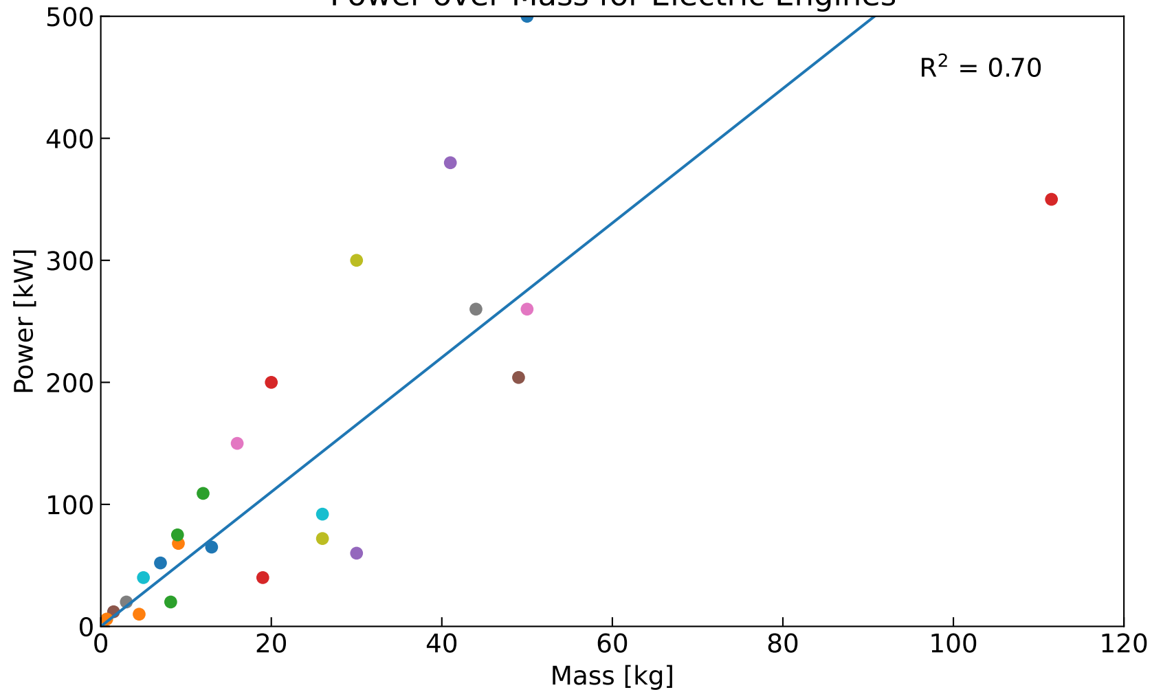
Power over Mass for Electric Engines
