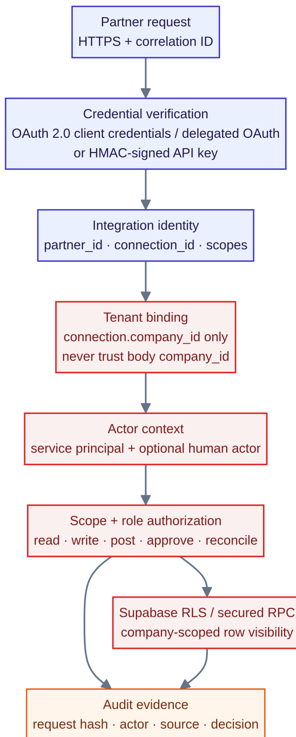
Figure 48: Enterprise Settings and Security Control Center evidence image from repository or captured application assets.
