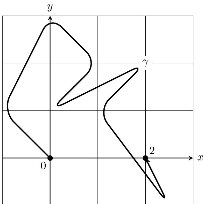
Figure 6.3: Seemingly complicated path integrals are easy to evaluate using the complex FTC. For the depicted contour, \int_{\gamma} e^z dz = e^2 - 1 .
