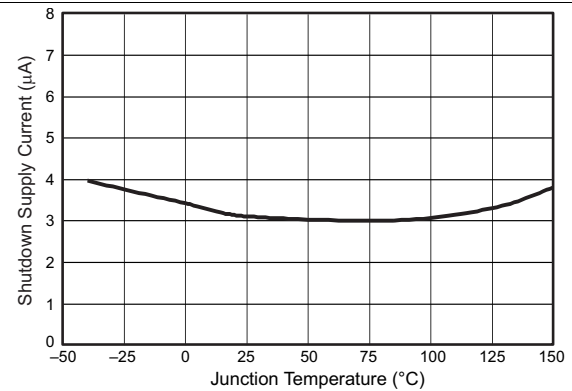
Figure 14. Shutdown Supply Current vs Temperature
