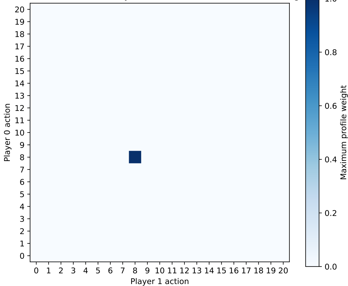
O2 — Linear Bertrand (symmetric): Maximum CE Profile Weight
