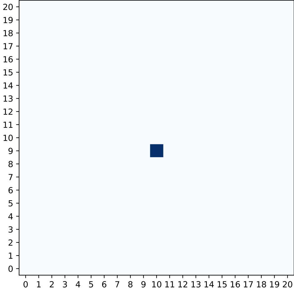
O2' — Linear Bertrand (asymmetric): Maximum CE Profile Weight
