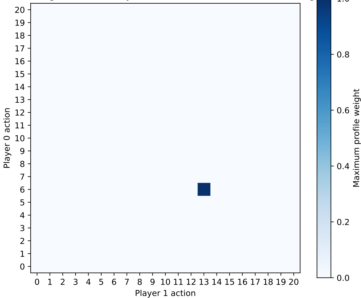
O3' — Logit Bertrand (asymmetric): Maximum CCE Profile Weight
