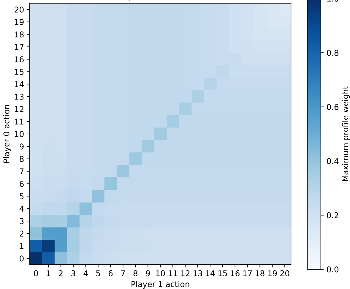
O1 — Standard Bertrand (symmetric): Maximum CCE Profile Weight
