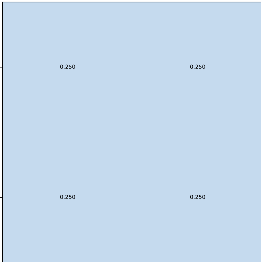
Matching Pennies: Maximum CCE Profile Weight
