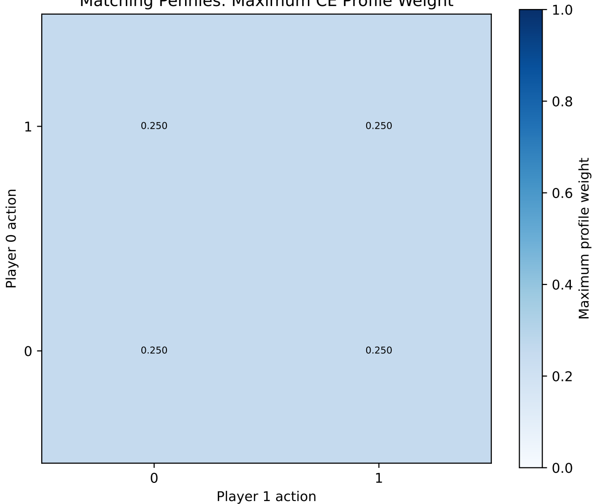
Matching Pennies: Maximum CE Profile Weight
