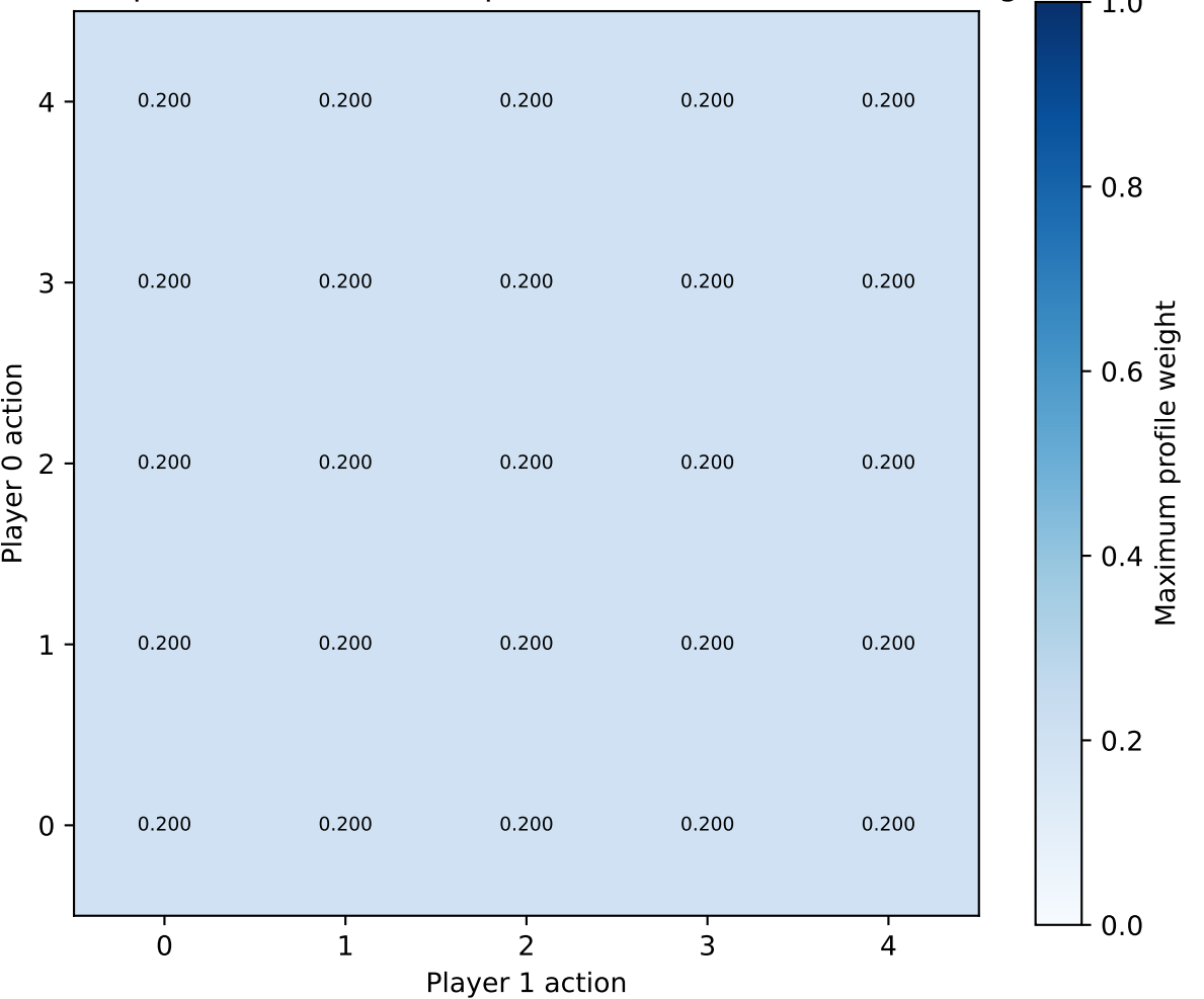
Rock-Paper-Scissors-Lizard-Spock: Maximum CCE Profile Weight
