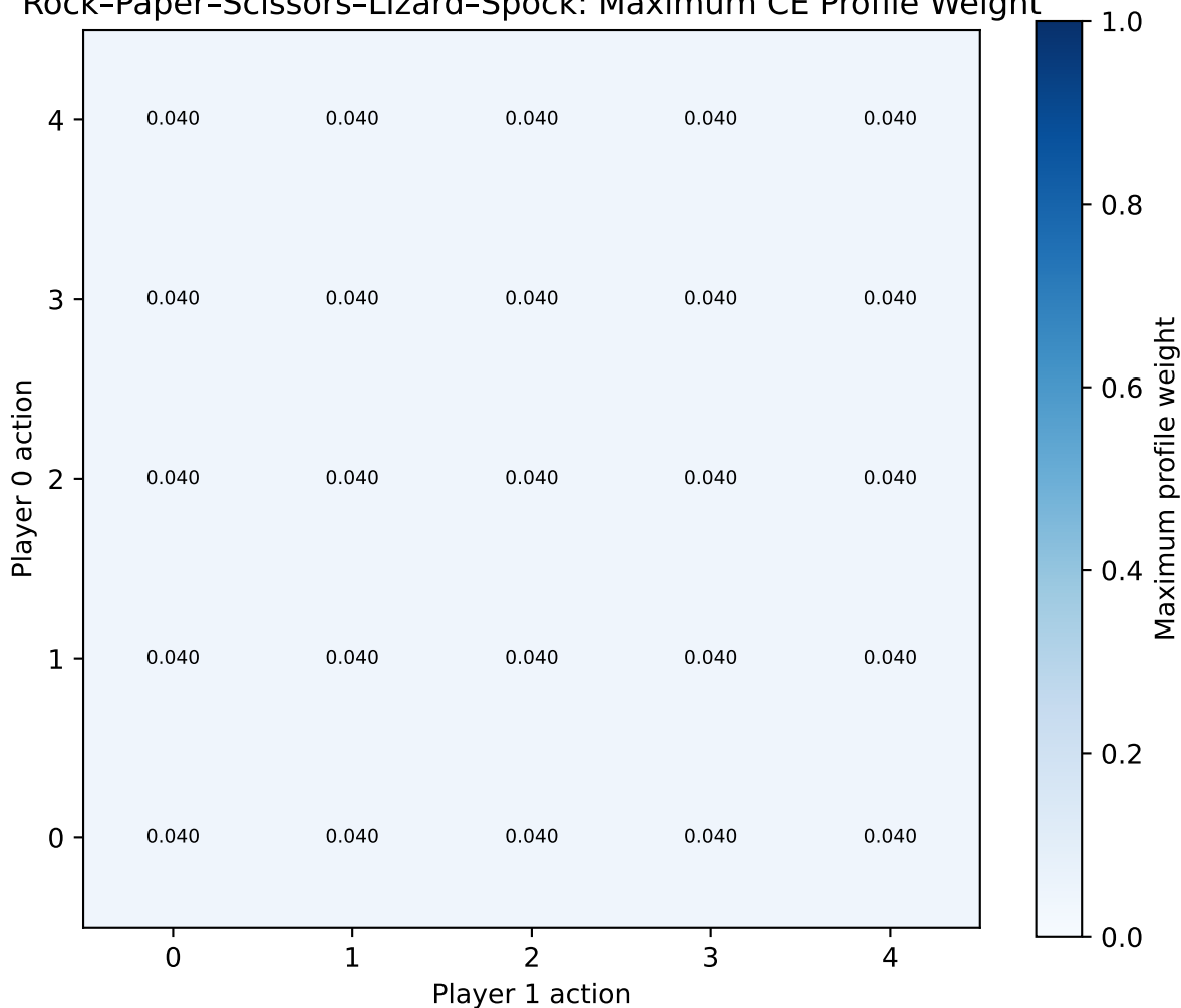
Rock-Paper-Scissors-Lizard-Spock: Maximum CE Profile Weight
