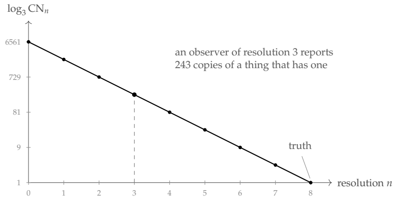
Figure 62.1: Proposition 62.3 for b = 3 , h = 8 ; the vertical axis is logarithmic, so the overcount is the vertical gap to the right-hand endpoint.
