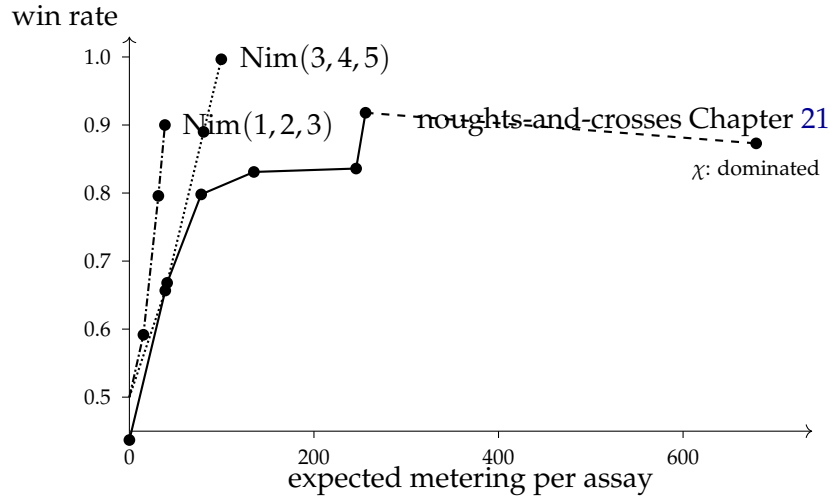
Figure 22.2: Three ladders on one pair of axes. The noughts-and-crosses curve turns down at its last rung—the complete theory costs more and wins less than the heuristic beneath it. Both Nim curves rise to the end, and the Nim(1,2,3) curve rises fastest at the top. Composition puts learners with curves of both shapes under one conserved \Theta .
