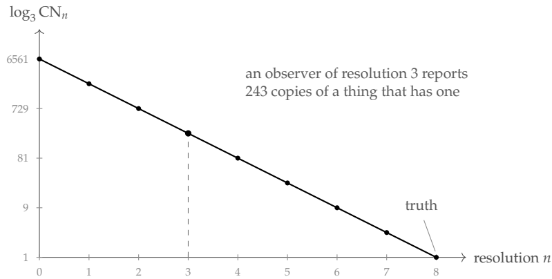
Figure 54.1: Proposition 54.3 for b = 3 , h = 8 ; the vertical axis is logarithmic, so the overcount is the vertical gap to the right-hand endpoint.
