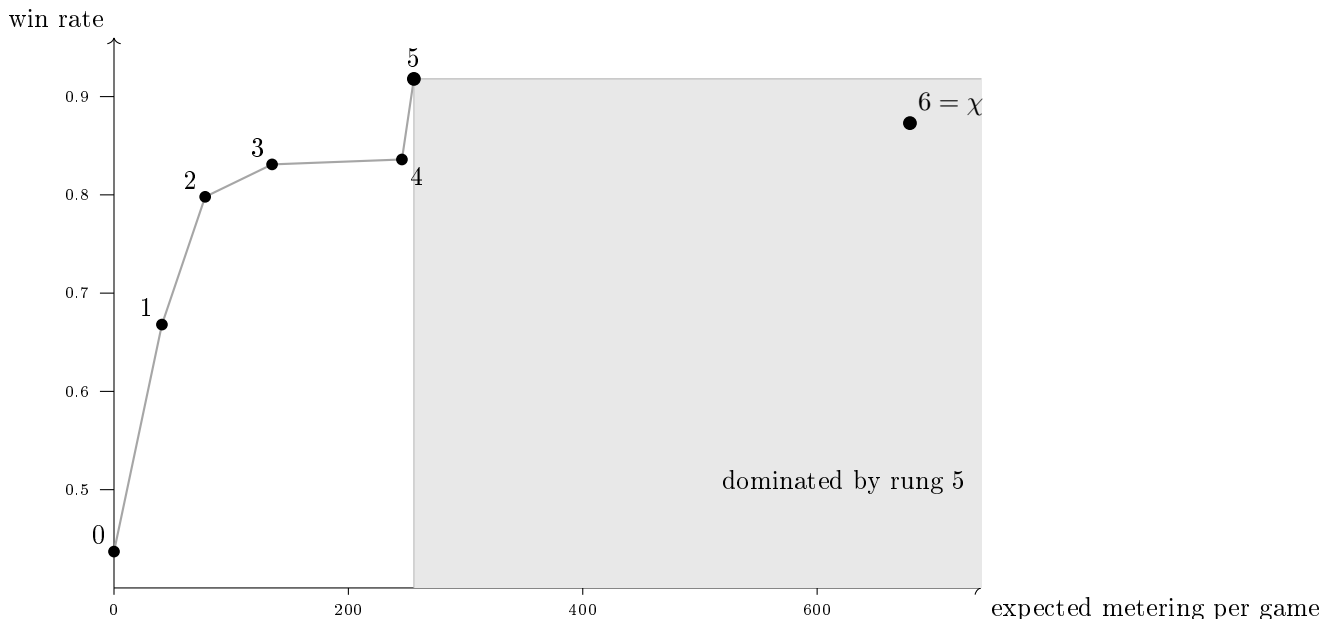
Figure 2: The ladder as a cost–yield curve, against a uniform-random opponent. Rungs 1–4 show sharply diminishing returns for a roughly doubling price, rung 4 —the alternating one—being the flattest. Rung 5, a predicate on square names of depth zero, is nearly free and delivers the largest jump on the ladder. The complete theory \chi lies inside the shaded region: it costs more than rung 5 and wins less, so it is dominated on both axes.
