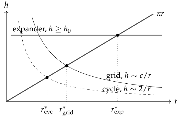
Figure 22.2: Individuation as a crossing. A region may be merged while its isoperimetric ratio lies above the line \kappa r , \kappa = \varepsilon\theta/\rho . Polynomially growing graphs cross early and give r^* \propto \kappa^{-1/2} ; an expander holds h up and crosses late, giving r^* \propto \kappa^{-1} and, since balls grow exponentially in r , an individual exponentially larger in population.
