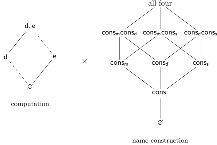
Figure 2: The expressive lattice, as a product of two independent axes over the base of \mathbf{m} and the routers. Nodes above \text{cons}_| carry it implicitly. Solid edges are strict by Propositions 9.5 and 9.9 and Corollary 9.6; dashed edges are Conjecture 9.10 and the open question of whether duplication alone adds anything in the absence of \mathbf{e} . The atoms \mathbf{q} , \mathbf{k} and \mathbf{fw} do not appear: on this ordering \mathbf{q} sits at the point of \mathbf{m} , and \mathbf{k} and \mathbf{fw} are derivable from the remaining routers (Propositions 9.11 and 9.12).
