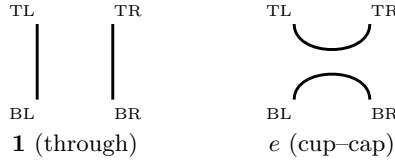
Figure 5: The two resolution-contexts of a gate-hole: the through-connector \mathbf{1} and the cup-cap e — the two diagrams of \text{TL}_2 . Kauffman’s relation reads \text{crossing} \mapsto A\mathbf{1} + A^{-1}e , and a closed loop of pure wire is worth \delta (so e^2 = \delta e ).
