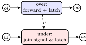
Figure 1: The crossing gate. The over-strand forwards its signal and produces the latch l ; the under-strand fires only on the join ( \& ) of its incoming signal with l . Chirality is exactly which strand produces l and which joins on it.
