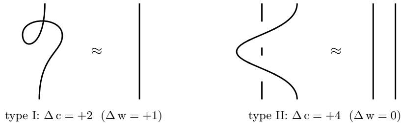
Figure 4: The two crossing-changing moves as local tangle equivalences. Left, type I: the kink and the bare strand are the same 1 \rightarrow 1 boundary forwarder; the kink adds one over-receive and one under-join, so \Delta c = +2 , which is 2 \Delta w . Right, type II: the over-passing bigon and the two parallel strands are the same 2 \rightarrow 2 forwarder; \Delta c = +4 , local and writhe-neutral. In both, the added machinery is internal ( \tau ), so weak bisimulation absorbs it.
