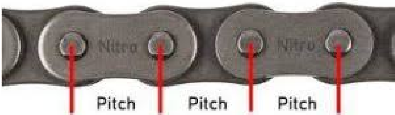
Measuring Roller Chain Pitch
