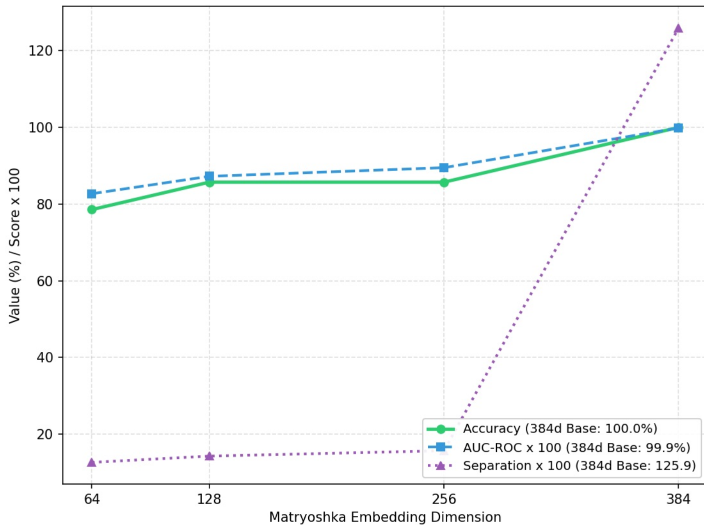
Absolute Performance vs. Dimension
