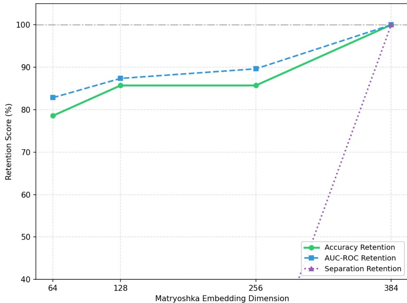
Relative Performance Retention (vs. 384d baseline)
