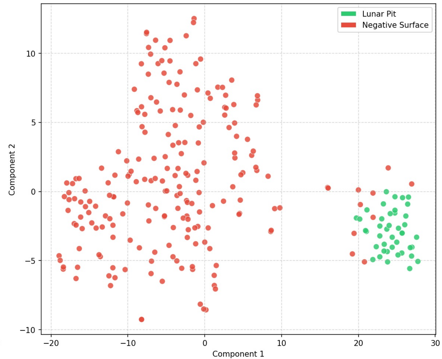
t-SNE Projection (384d space)
