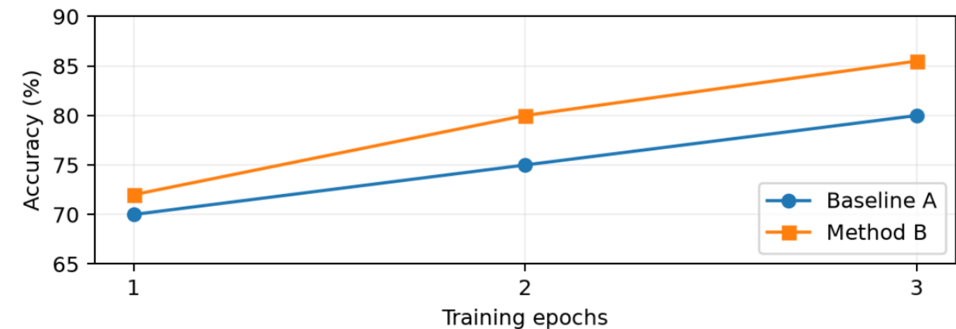
Figure 1. Test accuracy at three training epochs. Points are means.
