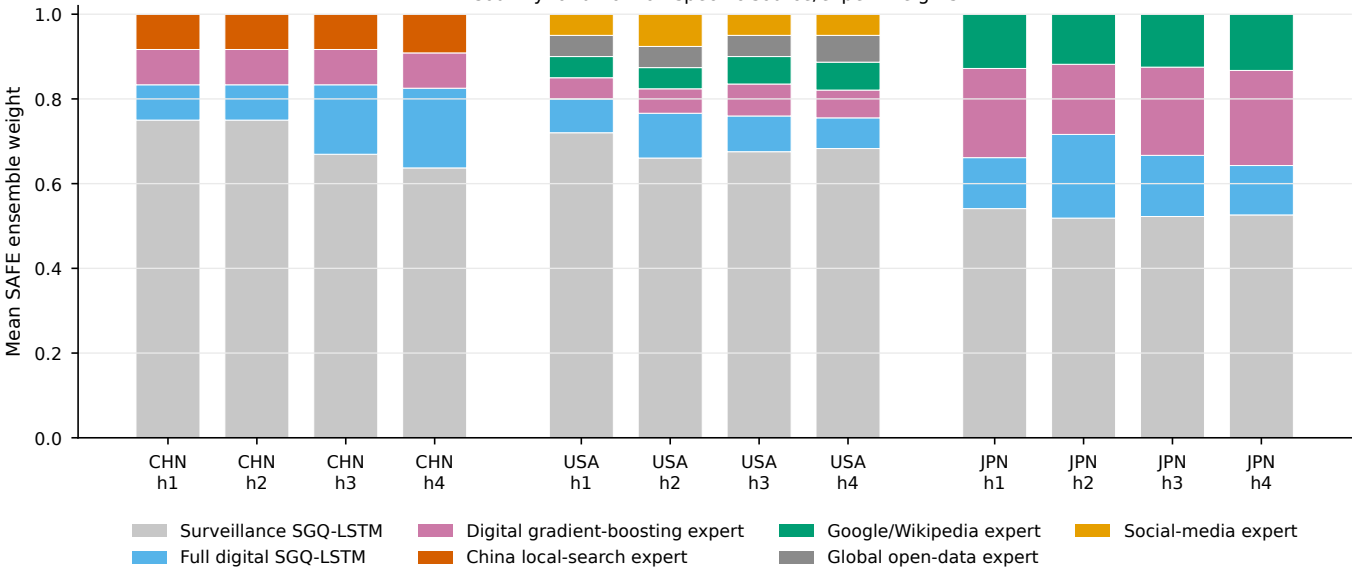
Country- and horizon-specific source/expert weights
