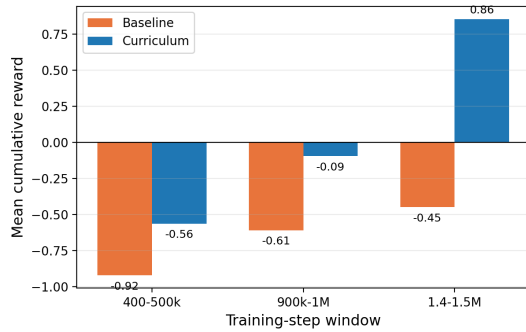
Figure 5: Mean cumulative reward at three step windows. The gap does not merely shift but widens ; by the final window the curriculum agent has crossed into positive reward (net success) while the baseline remains negative (net timeout).
