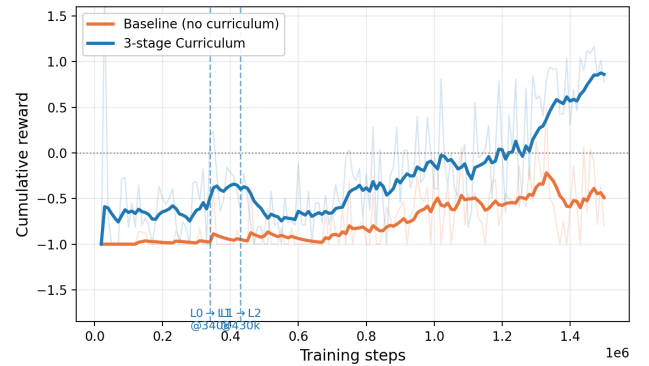
Figure 4: Cumulative reward over 1.5M training steps (faint: raw; bold: exponentially smoothed). The baseline (orange) plateaus near -0.5 , whereas the curriculum (blue) shows two inflection points at the lesson transitions—L0→L1 at 340k and L1→L2 at 430k steps—and then climbs steadily into positive reward.
