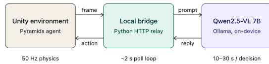
Figure 2: Diagram of VLM Agent Architecture
