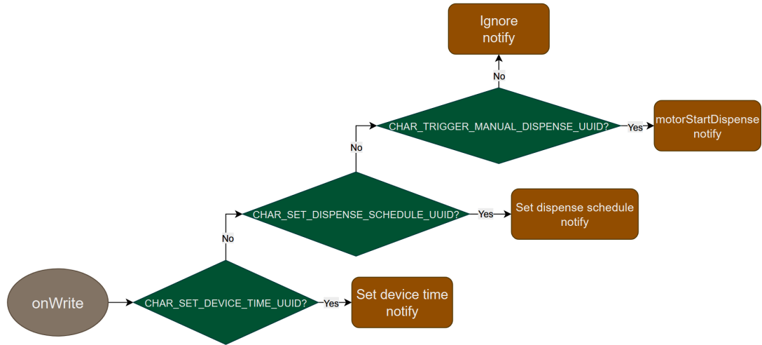
Figure 15: Flowchart of the onWrite method of MyCharacteristicCallbacks class shows the logic under which this method operates. Notify means that whoever was subscribed to updates to a certain Characteristic will get a signal that the value has changed.
