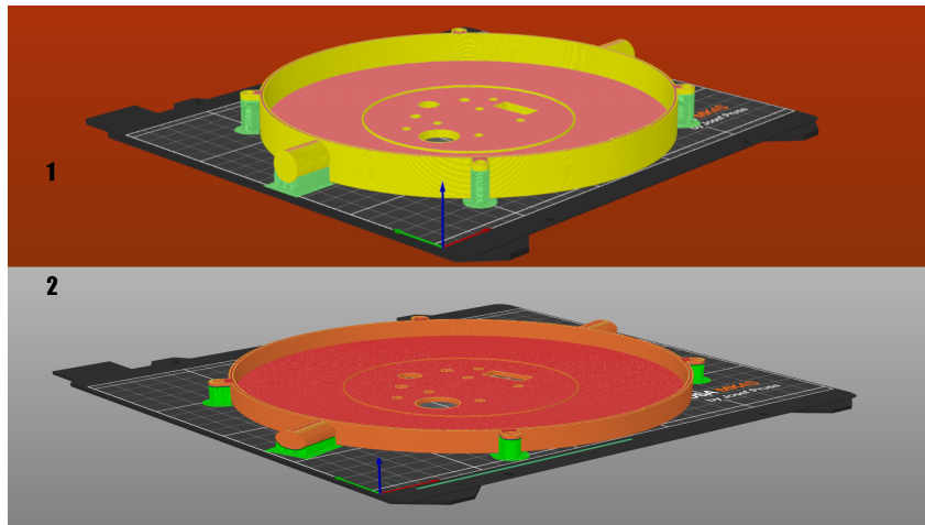
Figure 12: Issue when slicing. On the upper image (1) the supports are out of printing bounds, as the ominous red aura highlights at this problem. On the lower image (2) the problem is fixed. The component was rotated, so that the sticking-out parts of it are given a certain distance from the border to be able to draw support material
