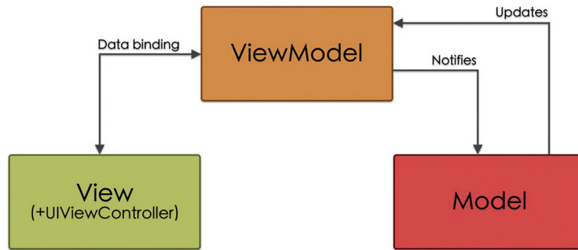
Figure 16: Model-View-ViewModel Structure. This Figure explains what model consists of and how different parts of model interact with each other. Credit [26]
