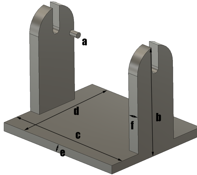
Figure 11: Stand. (a) is the notch to prevent backwards tilting. (b) measurement from bottom to the peak. (c) Stand width. (d) Length.(e) Floor thickness. (f) Pillar thickness
