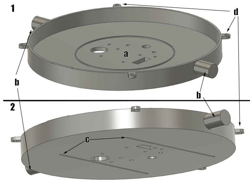
Figure 8: Lower Body. (1) view from above. (2) view from below. (a) depicts inner area for cutouts to connect electronics that are directly connected to Lower Body. (b) depicts hoisting "ears". (c) grooves for Lower Deck. (d) connectors that bind Lower Body to Upper Body
