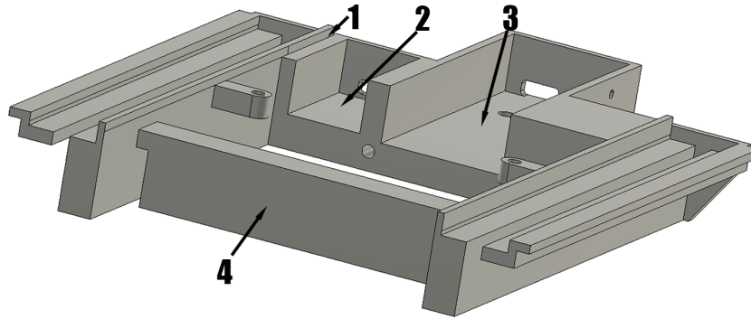
Figure 10: Lower Deck and its' features: (1)Ridge (2)Microcontroller housing (3)Charger Module housing (4)Battery Wall
