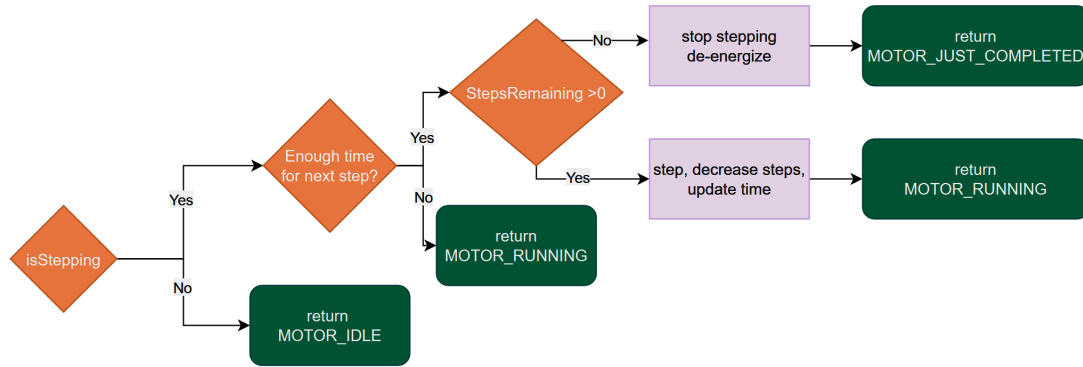
Figure 13: The flow chart of stepper motor control logic within the motorLoop() function. This function is called repeatedly within loop() function of the main.cpp file.
