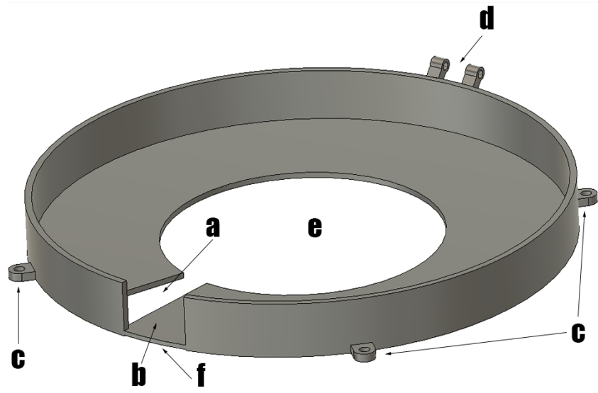
Figure 5: Upper Body of the Pill Dispenser. (a) shows the cutout for the disposal pathway. (b) shows the cutout for dispense pathway. (c) shows the connectors which will connect Upper Body and Lower Body together using screws. (d) shows the connector for the lid of the device (e) shows the housing of the Mills. (f)
