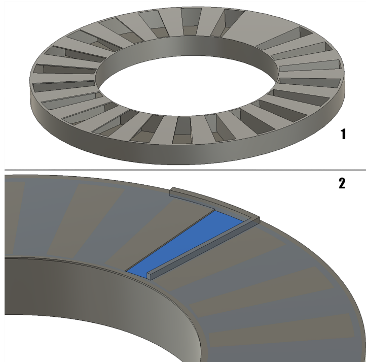
Figure 4: Decomposed Disposal mechanism of 2nd revolver system. (1) Shows the Lower Mill without cover. the whole construction would be rotating, covered by a ring with a cutout, seen on (2)
