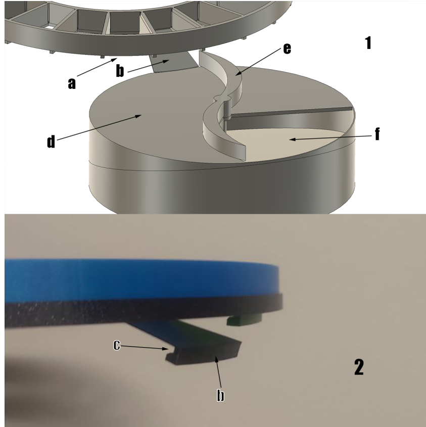
Figure 2: First revolver prototype. Seen here, the initial idea was to have a trapdoor in each chamber which will release the pills onto the disposal dish by opening it. (1) Is a designed prototype, (2) is a photo of 3D-printed prototype. (a) Depicts a chamber. (b) Door. (c) Notch for the lever to open the door. (d) Dispensing ramp. (e) S-shaped arm. (f) Disposal ramp
