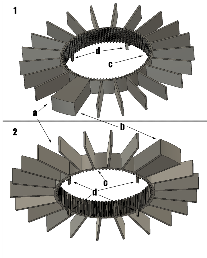
Figure 6: Upper Mill. (1) View from above. (2) view from below. (a) shows 1 of 21 functional chambers. (b) service chamber. (c) gears on the inner rim. (d) connector teeth.
