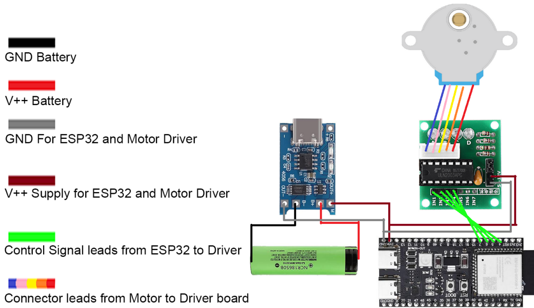
Figure 9: Connection schema of electronic components. Components from top to bottom: 1)28BYJ Stepper motor 2) Left: Charger Module 3)Right: ULN2003 Motor Driver 4)Left:Panasonic NCR18650B Battery 5)Right ESP32 S3 DevKitC-1 N16R8 S3 Micro-controller
