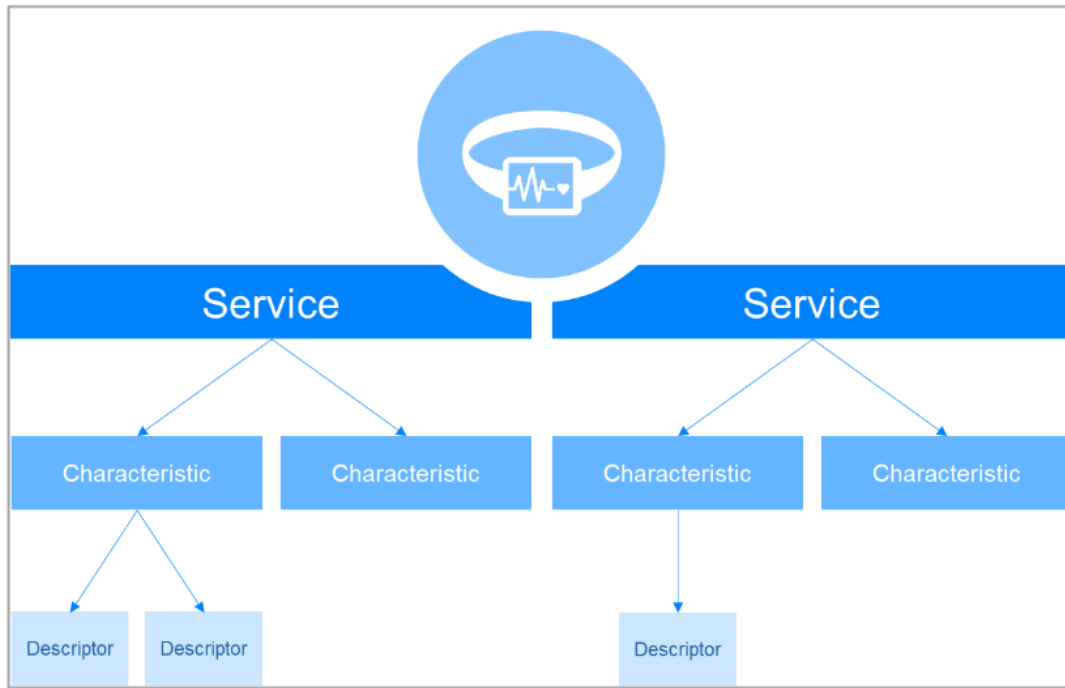
Figure 14: Generic Attribute Profile hierarchy shows the structure of service, characteristics and descriptors. Credit [15]
