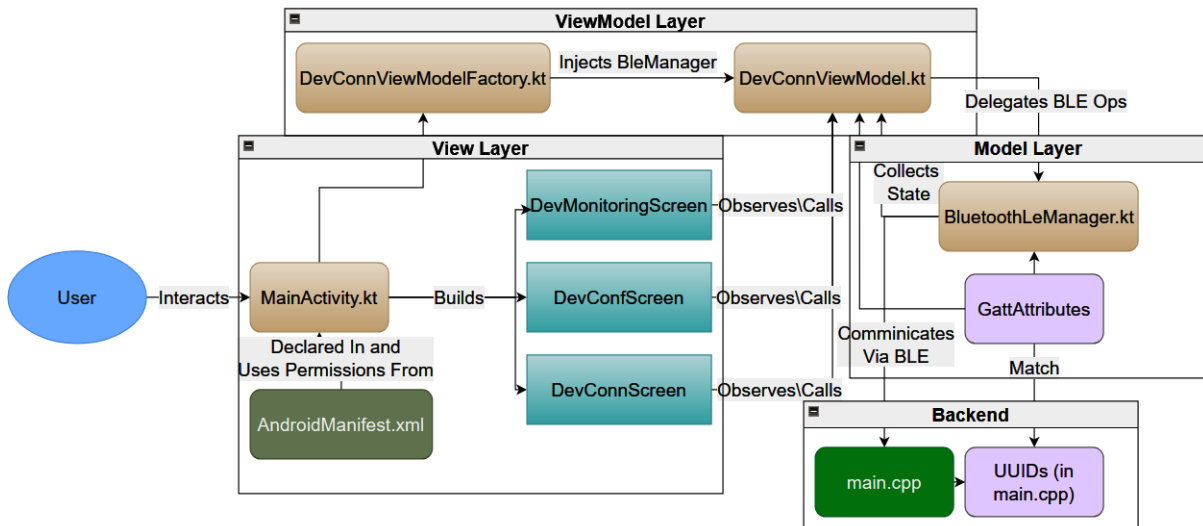
Figure 17: Diagram of an Android App showing how its different components interact with each other and with backend. The structure is divided into 3 parts: View Layer, ViewModel Layer and Model Layer, corresponding to MVVM paradigm.
