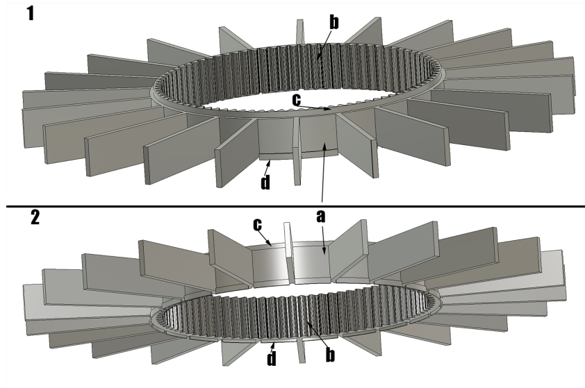
Figure 7: Lower Mill. (1) view from above. (2) view from below. (a) depicts chambers. (b) cogs of the inner rim. (c) antifriction ring at the top. (d) antifriction rims at the bottom
