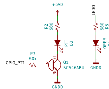
LEDs
