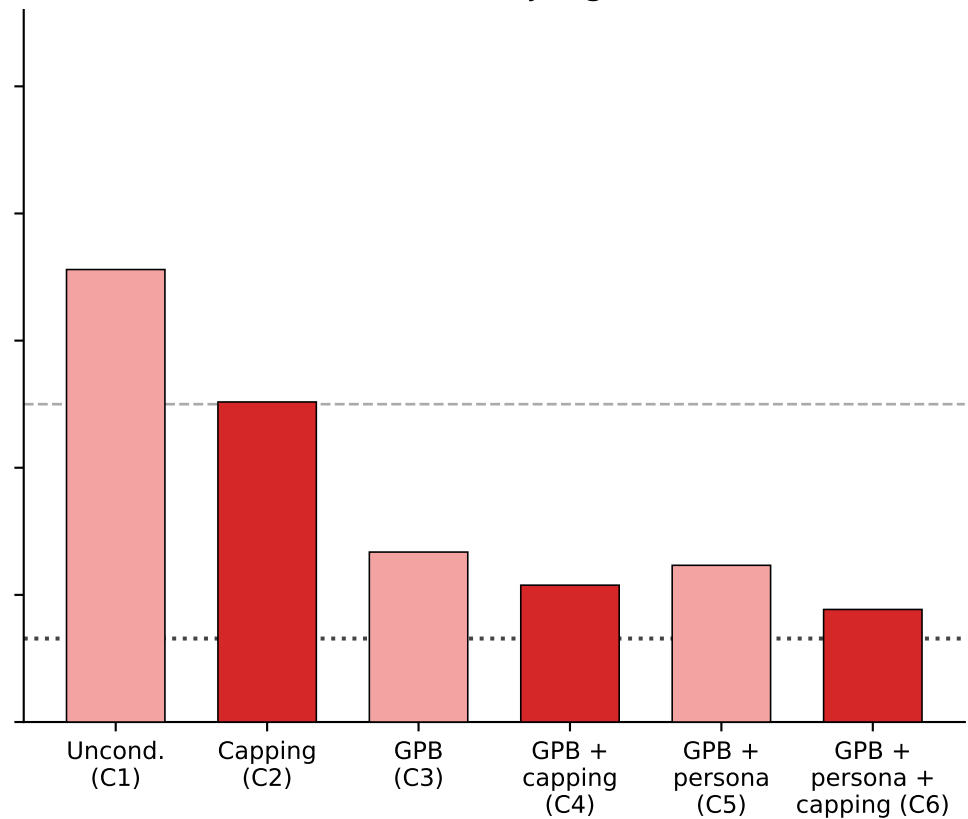
Erroneous judges
