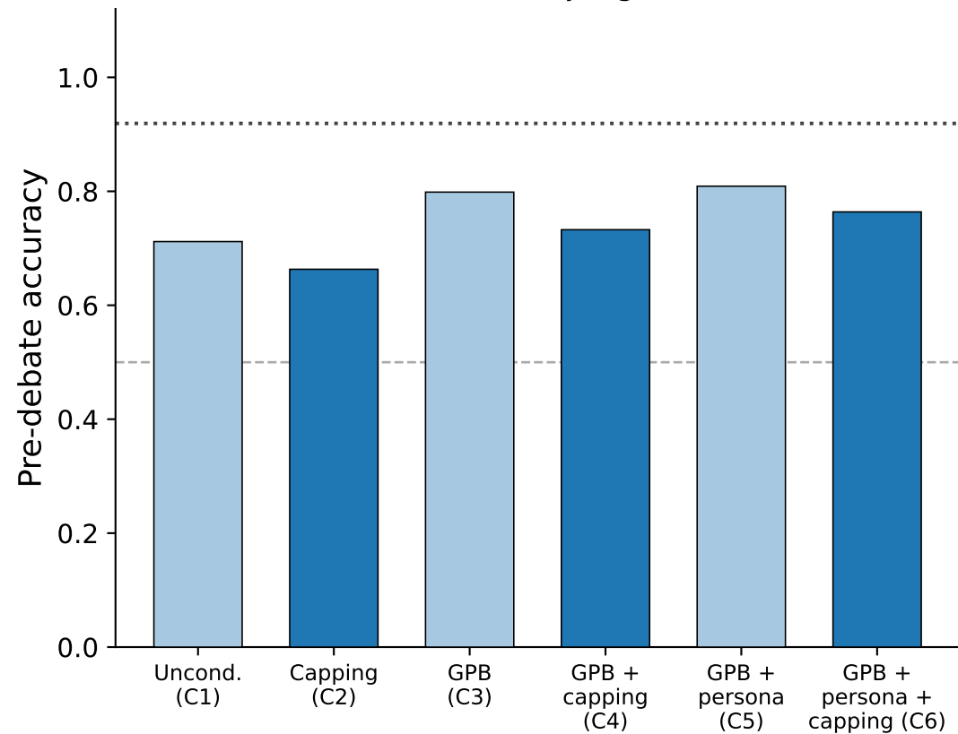
Grounded judges
