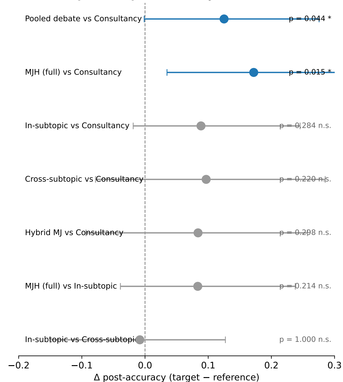
B. Cross-protocol post-accuracy contrasts (95% CI)
