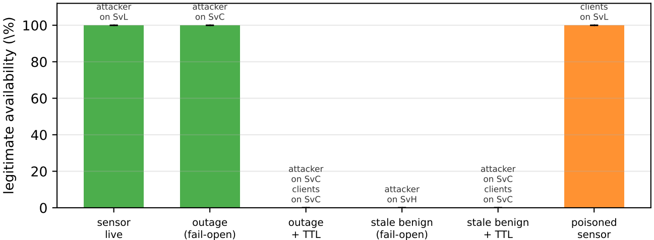
Legitimate availability under Slowloris across sensor failure modes
