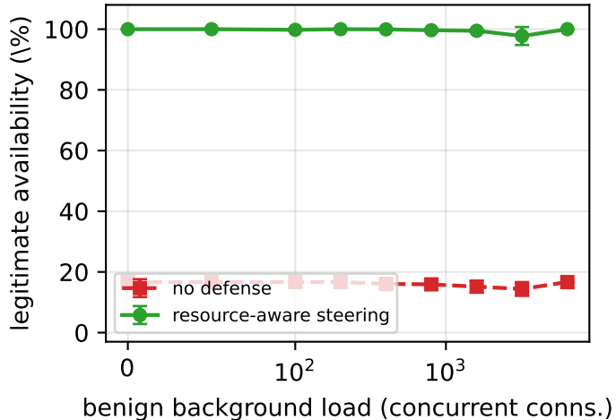
(a) legitimate-workload scale
