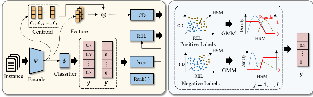
Figure 4: The overall framework of LeD. \hat{y} represents the predicted labels, \tilde{y} denotes the observed labels, and \check{y} stands for the corrected pseudo-labels. CD refers to the centroid distance, REL stands for ranking-enhanced loss, and HSM denotes the holistic selection metric.
