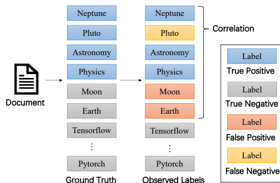
Figure 1: An illustration of noisy multi-label text classification.
