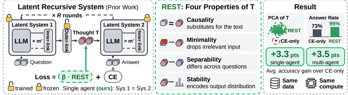
Figure 1. Overview of REST. Latent systems pass a thought T through a trained outer link (left). REST adds a \beta -weighted loss built from the four properties of T to the CE objective (middle). CE-only thoughts collapse and REST improves accuracy under the same data and compute (right).
