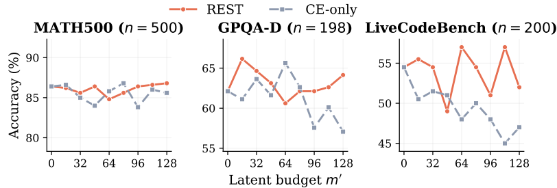
Figure 12. Accuracy against the latent budget m' for the Scaled system at r = 1 .
