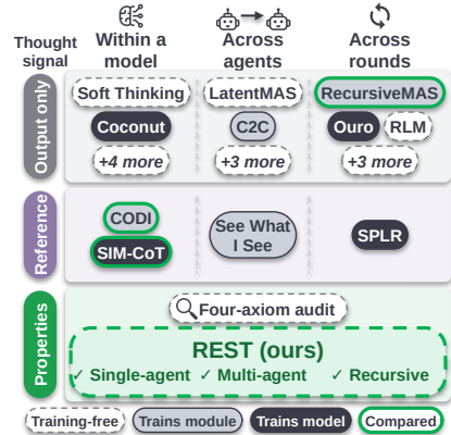
Figure 7. Positioning of REST.
