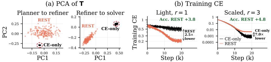
Figure 6. REST against CE-only. (a) PCA for \mathbf{T} . CE thoughts collapse into dense clusters, while REST spreads thoughts apart. (b) Training CE under causality. More details in Appendix D.
