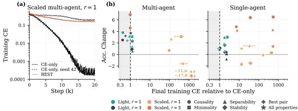
Figure 11. Training CE. (a) Training CE loss for causality at \beta = 3.0 . (b) Mean of last CE 200 steps relative to CE-only against Acc. Change. Bars span seeds.
