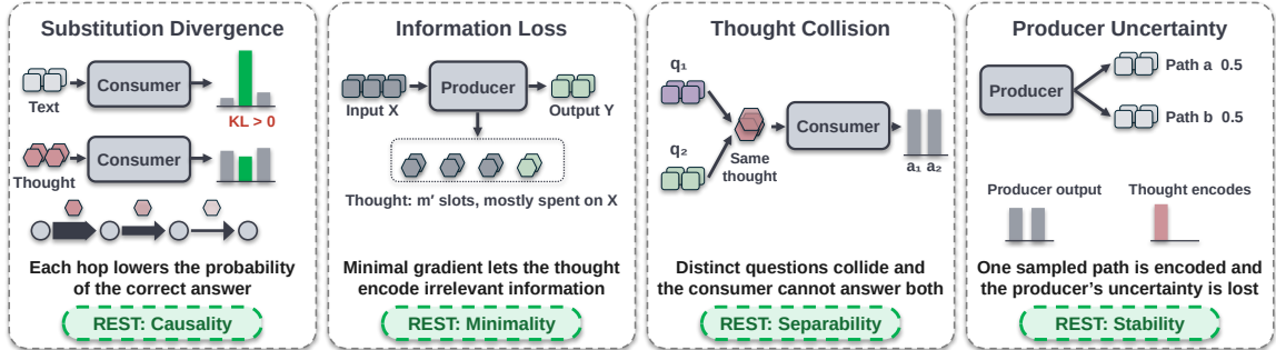
Figure 2. Why CE is not enough. Four failures of CE thoughts and the property that addresses each.
