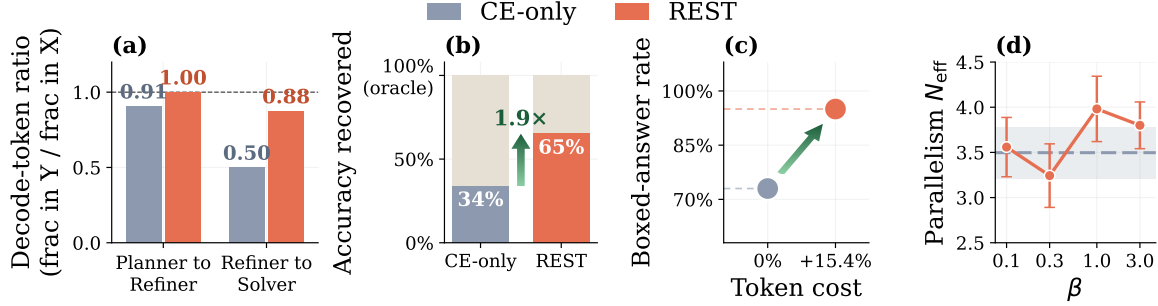
Figure 5. REST against CE-only. (a) Decoded thoughts compared to output / input. (b) Replacing oracle text with thought. (c) Answer rate vs token usage. (d) Effective Superposition.
