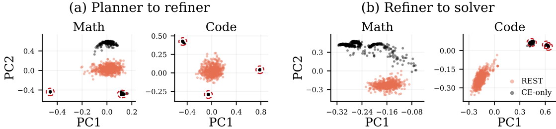
Figure 10. PCA for T. CE thoughts collapse into dense clusters, where each dashed ring holds all questions of one training run, while REST spreads thoughts apart.
