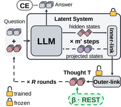
Figure 3. Single agent. \mathcal{R}_{in} runs at each of the m' steps, and \mathcal{R}_{\psi} once per round.
